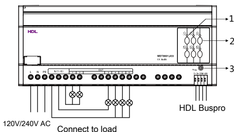
Figure 4. Wiring
