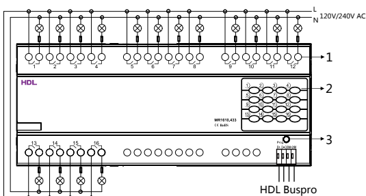
Figure 4. Wiring
