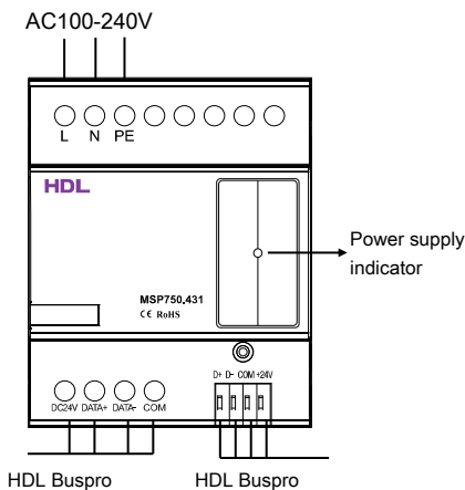
Figure 4. Wiring
