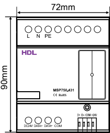
Figure 2. Dimensions - Front View
