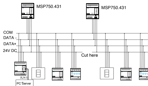
Figure 5. Wiring
