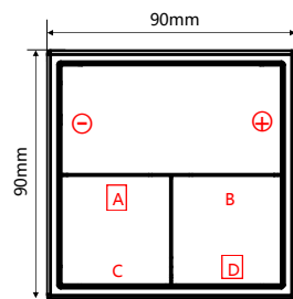
Figure 3. Dimensions - Metal version
