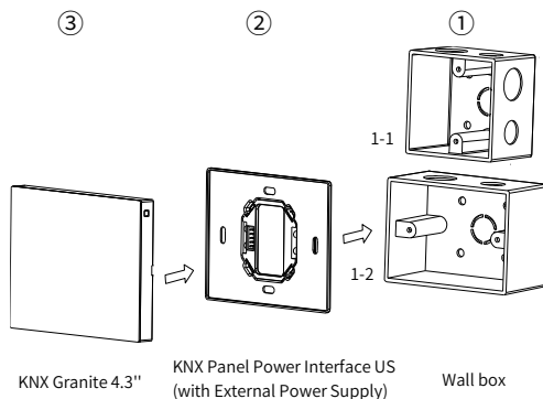
Figure 10. Landscape Installation
