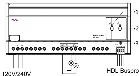
Figure 4. Wiring
