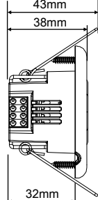
Figure 3. Dimensions - Side View
