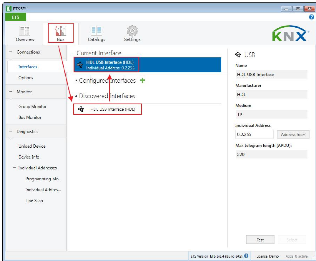
Figure 14- 1 Interface setting
