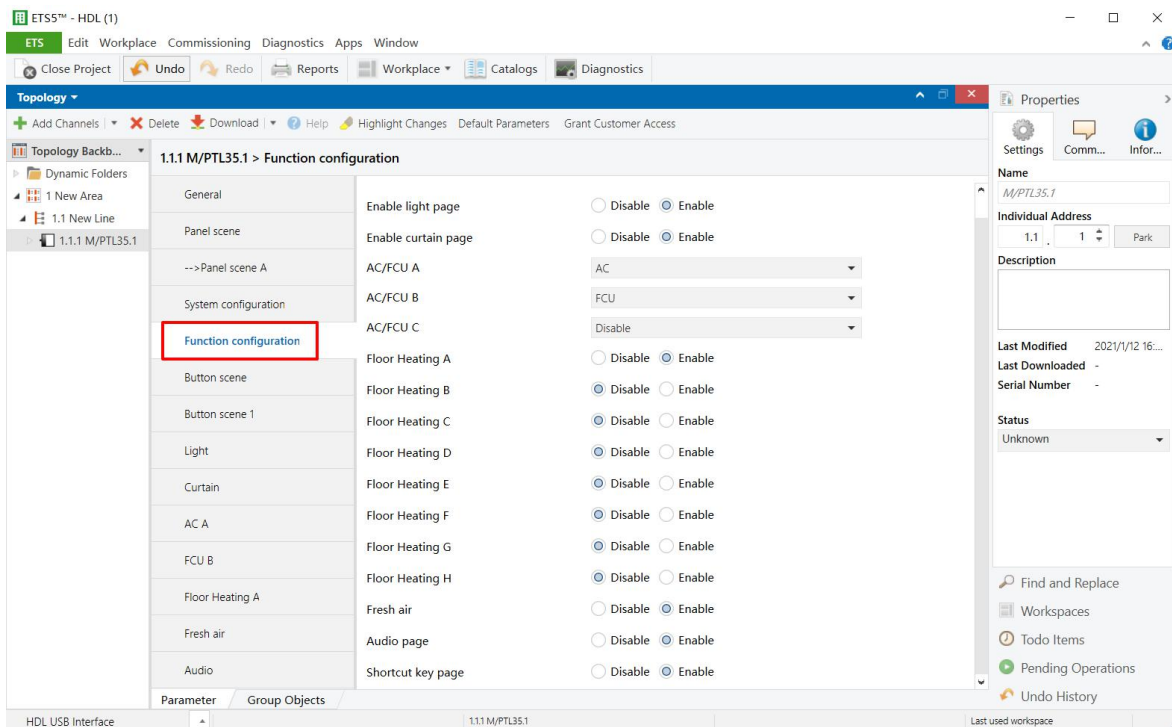
Figure 5- 1 Function setting
