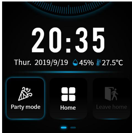
Main page
