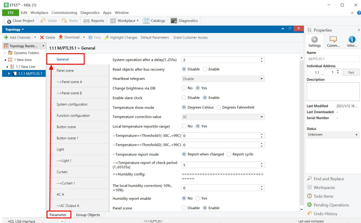
Figure 2-1 General setting
