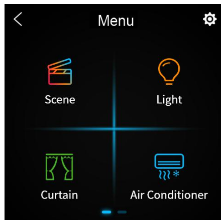
Main menu
