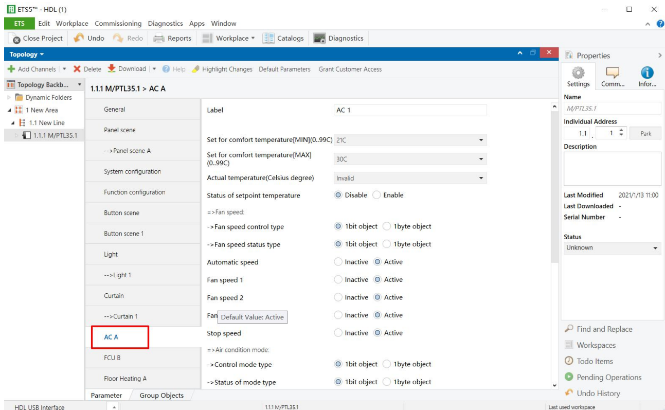
Figure 9-2 AC settin
