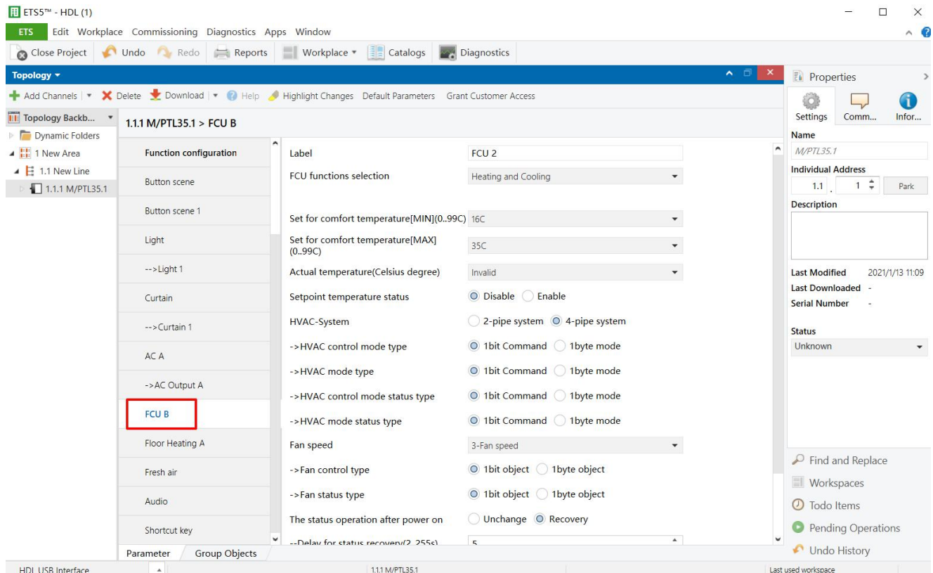
Figure 9-4 FCU setting
