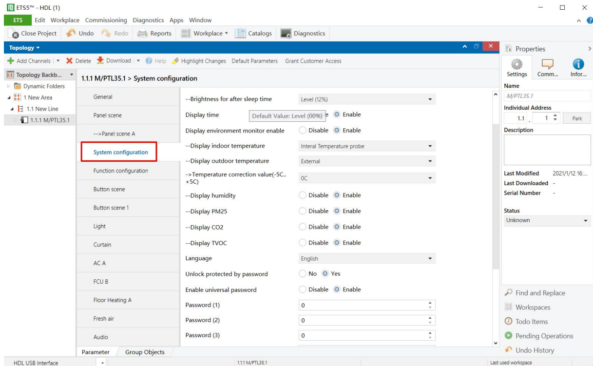
Figure 4- 1 System setting
